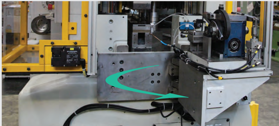
TAB ROLL FEED APRON: Opened position for pull out tap tool
